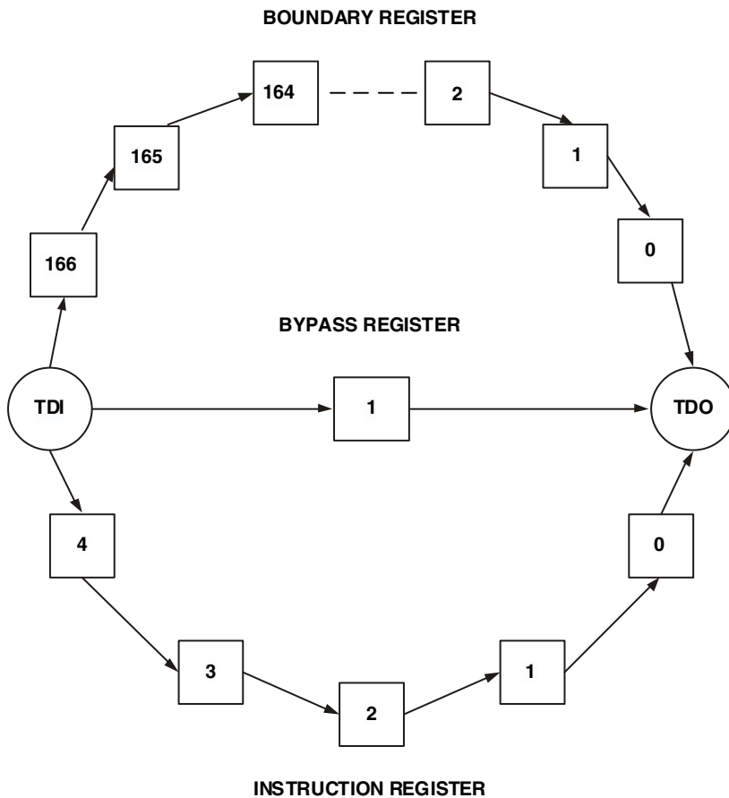
Figure 6-1. Serial Scan Path
