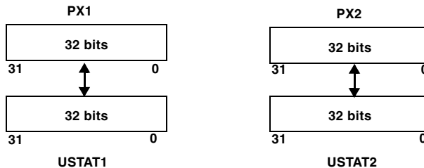
Figure 5-6. Transfers Between USTATx and PX Registers
