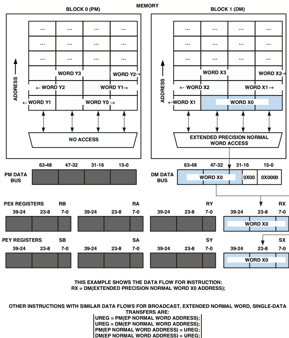
Figure 5-31. Extended-Precision Normal Word Addressing of Single-Data in Broadcast Load
