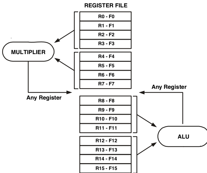
Figure 9-4. Permitted Input Registers for Multifunction Computations
