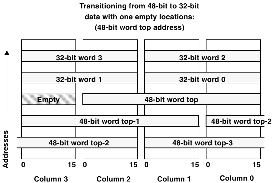
Figure 5-9. Mixed Instructions and Data With One Unused Location
