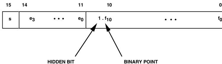
Figure 2-4. 16-Bit Floating-Point Format
