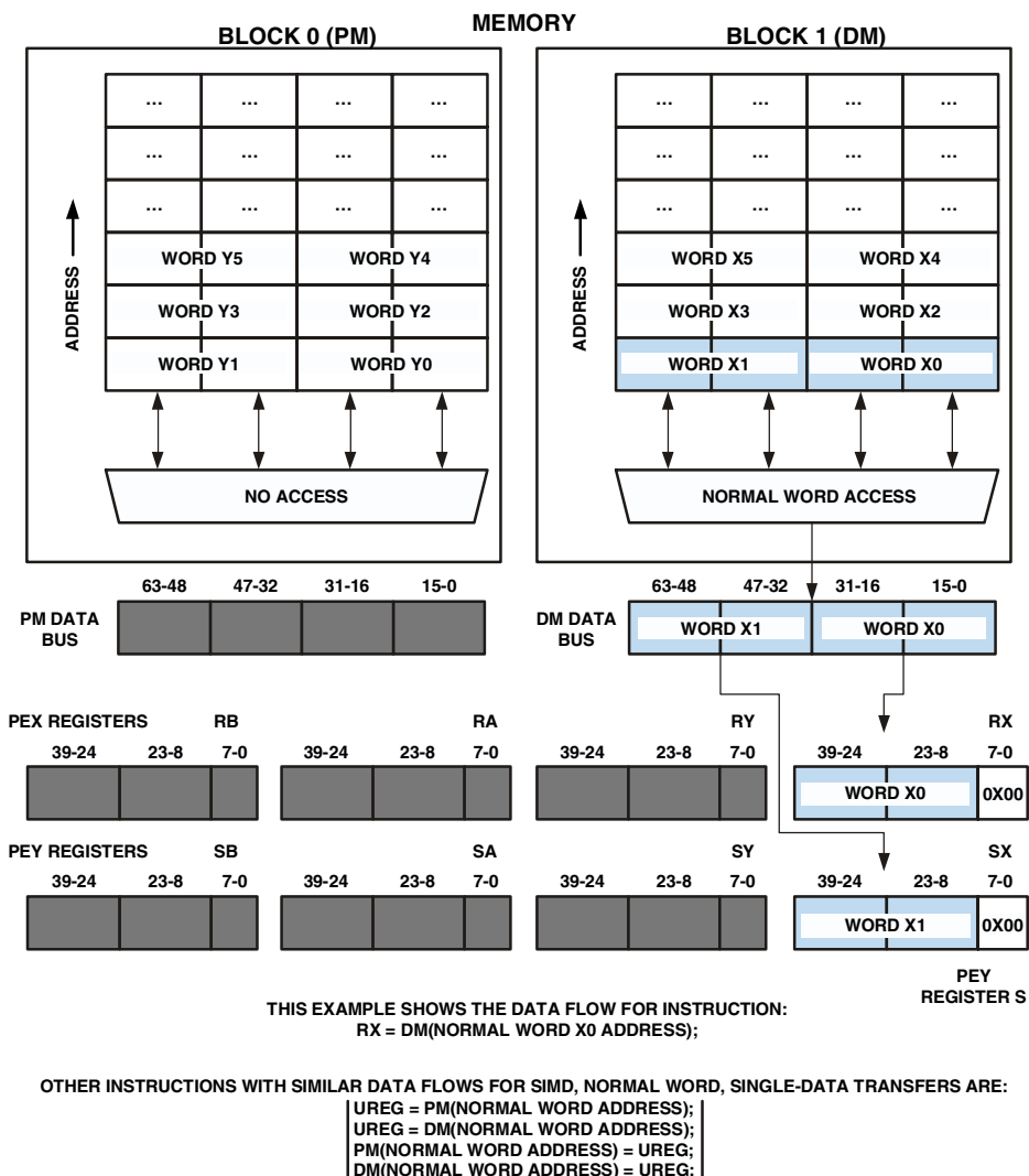
Figure 5-16. Normal Word Addressing of Single-Data in SIMD Mode
