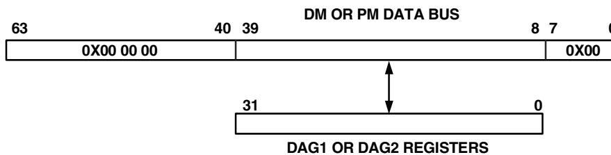
Figure 4-7. DAG Register-to-Data Register Transfers
