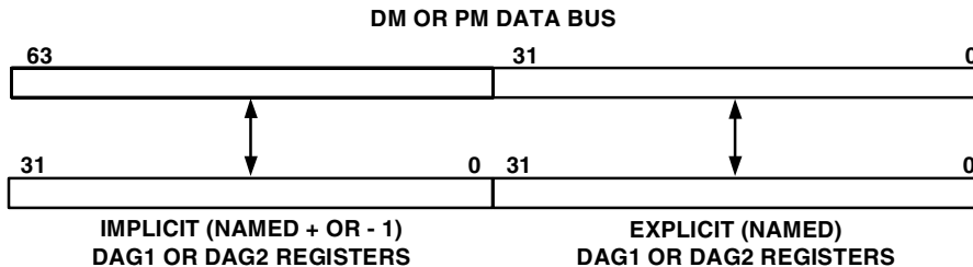
Figure 4-8. Long Word DAG Register-to-Data Register Transfers
