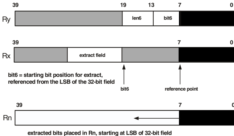
Figure 9-3. Field Alignment
