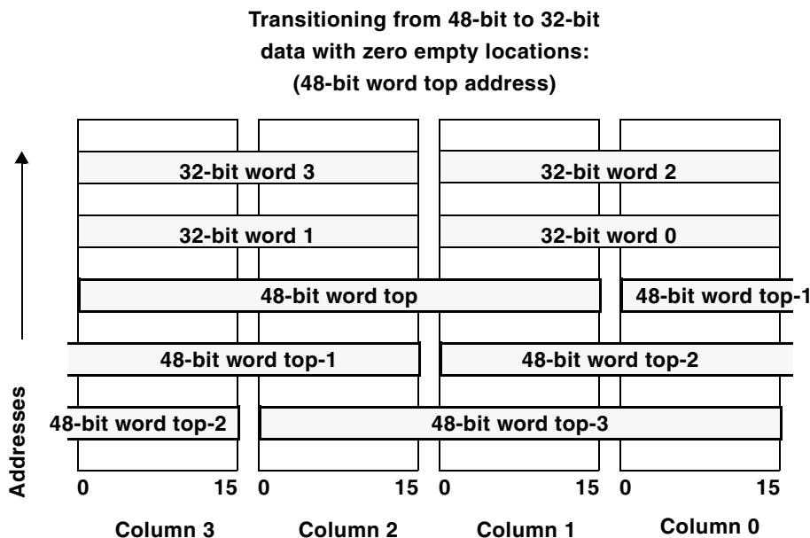
Figure 5-8. Mixed Instructions and Data with No Unused Locations
