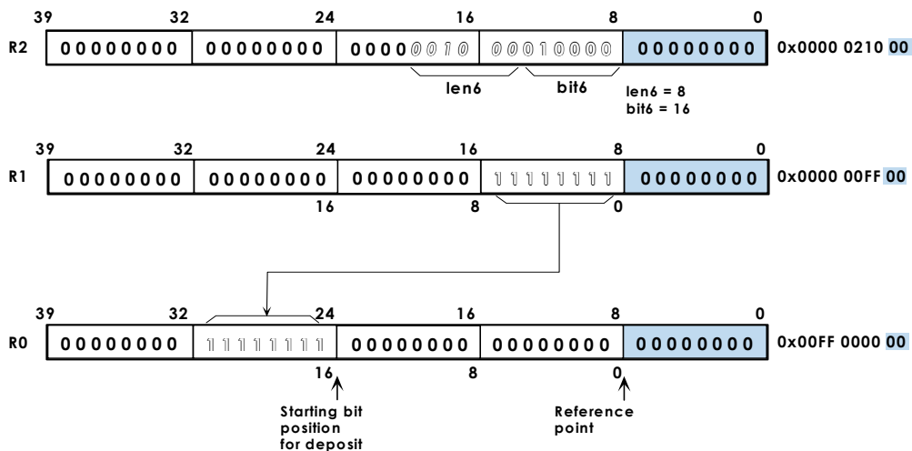
Figure 2-12. Bit Field Deposit Instruction
