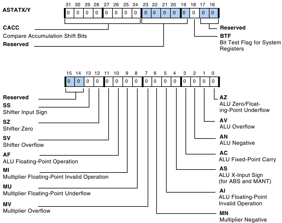
Figure B-6. ASTAT Register
