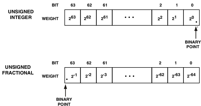
Figure 2-6. 64-Bit Unsigned Fixed-Point Product
