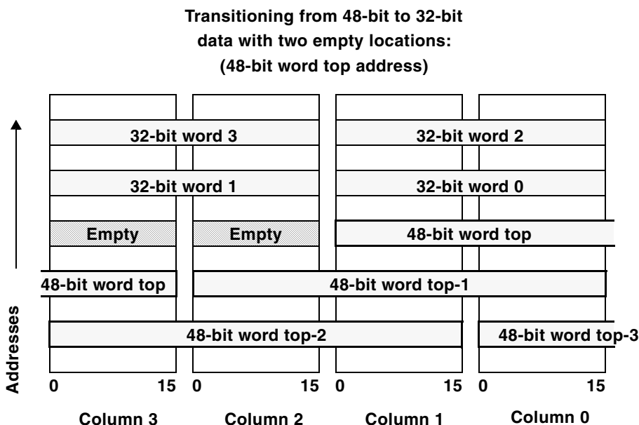
Figure 5-10. Mixed Instructions and Data With Two Unused Locations
