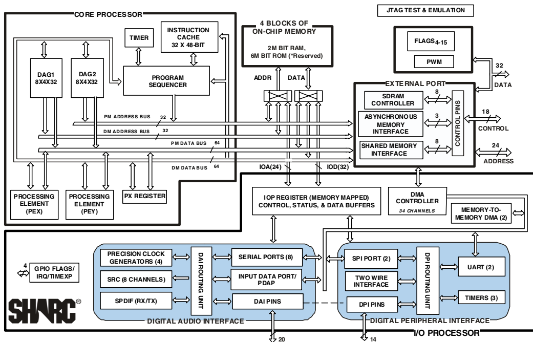
Figure 1-2. ADSP-21367/8/9 SHARC Processor Block Diagram
