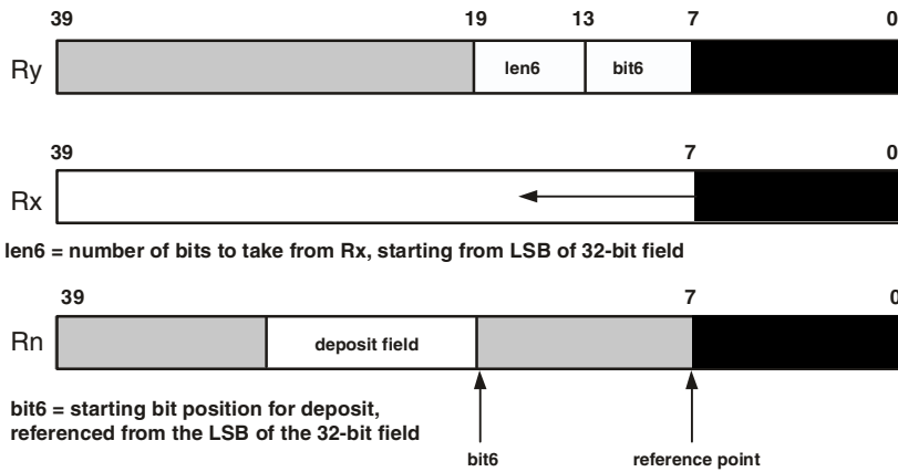
Figure 9-1. Field Alignment
