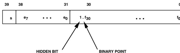
Figure 2-3. 40-Bit Extended-Precision Floating-Point Format
