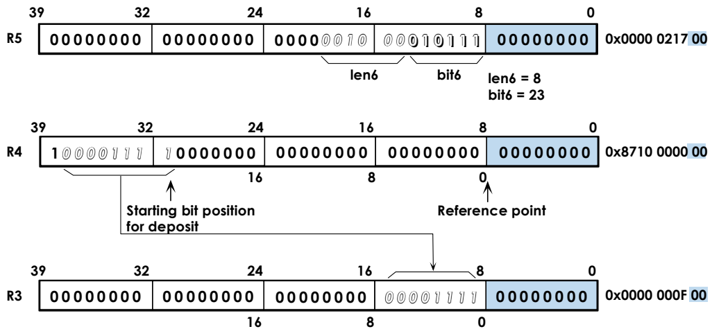
Figure 2-14. Bit Field Extract Instruction
