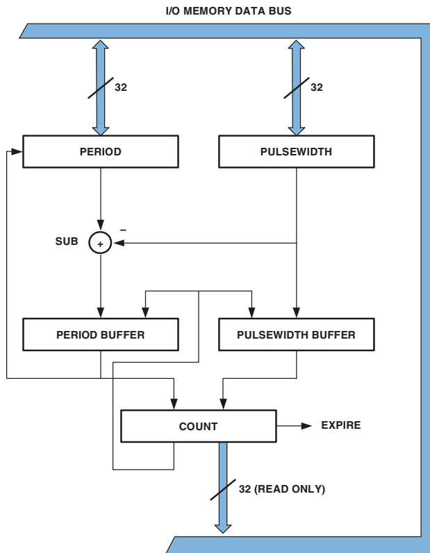
Figure 7-1. Timer Block Diagram
