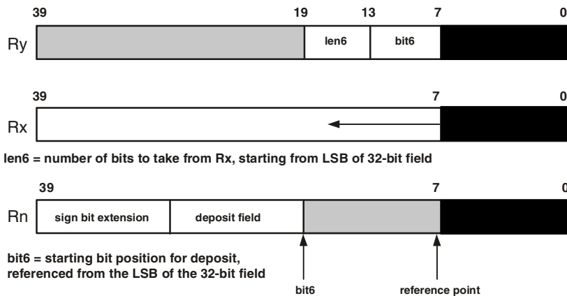
Figure 9-2. Field Alignment
