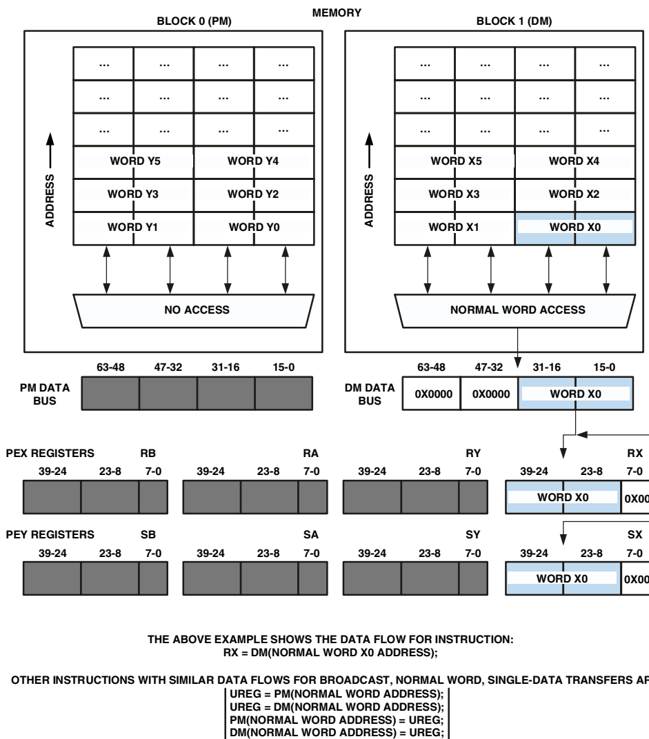
Figure 5-29. Normal Word Addressing of Single-Data in Broadcast Load
