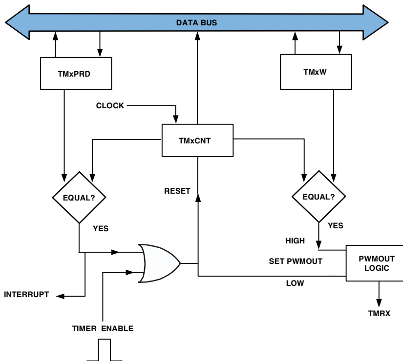
Figure 7-4. Timer Flow Diagram – PWM_OUT Mode
