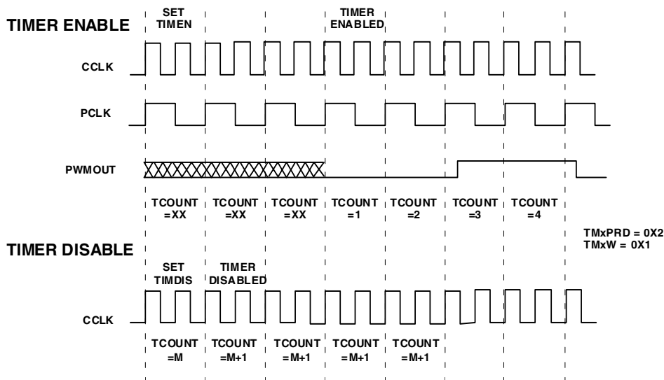
Figure 7-3. Timer PWM Enable and Disable Timing
