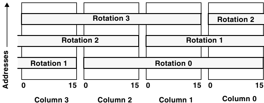
Figure 5-7. 48-Bit Word Rotations
