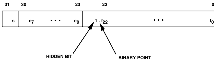
Figure 2-2. IEEE 32-Bit Single-Precision Floating-Point Format
