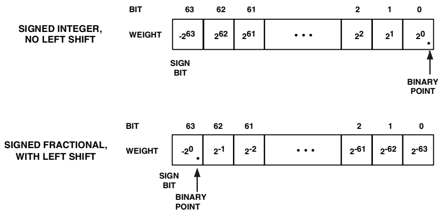
Figure 2-7. 64-Bit Signed Fixed-Point Product
