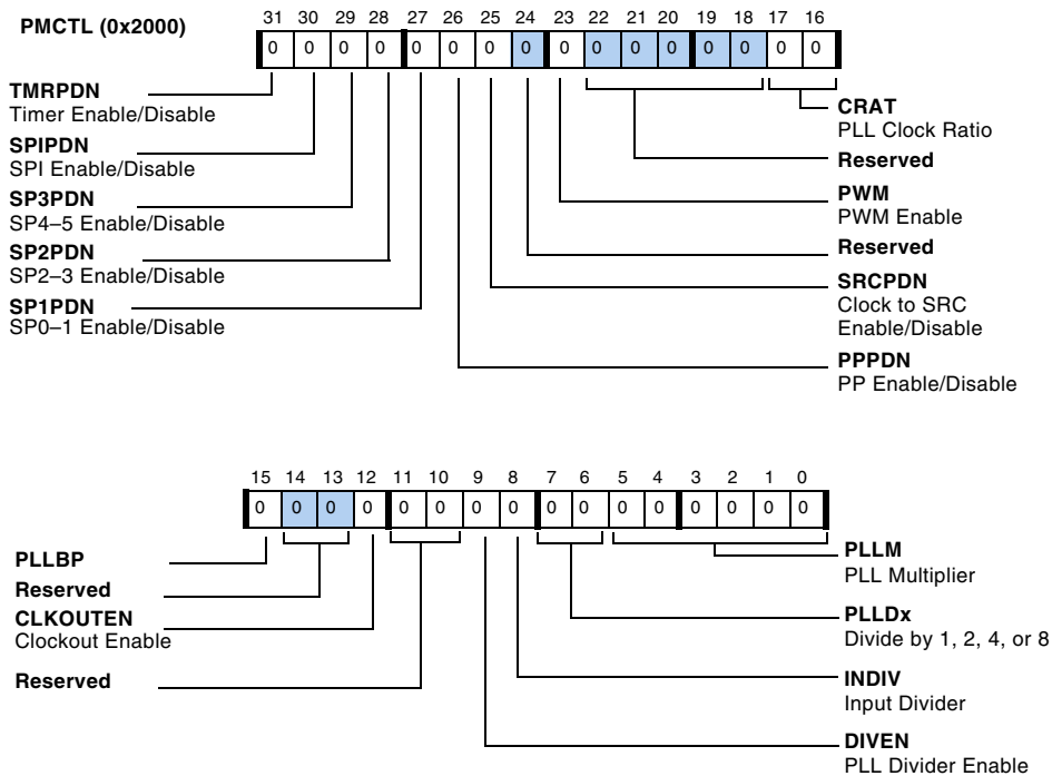
Figure B-14. PMCTL Register
