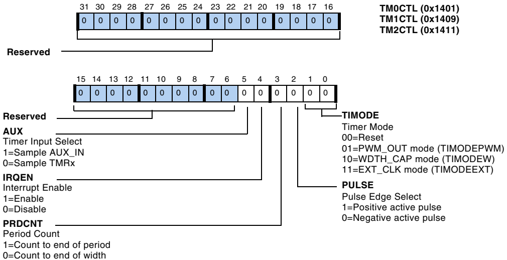
Figure B-12. Timer Configuration Register
