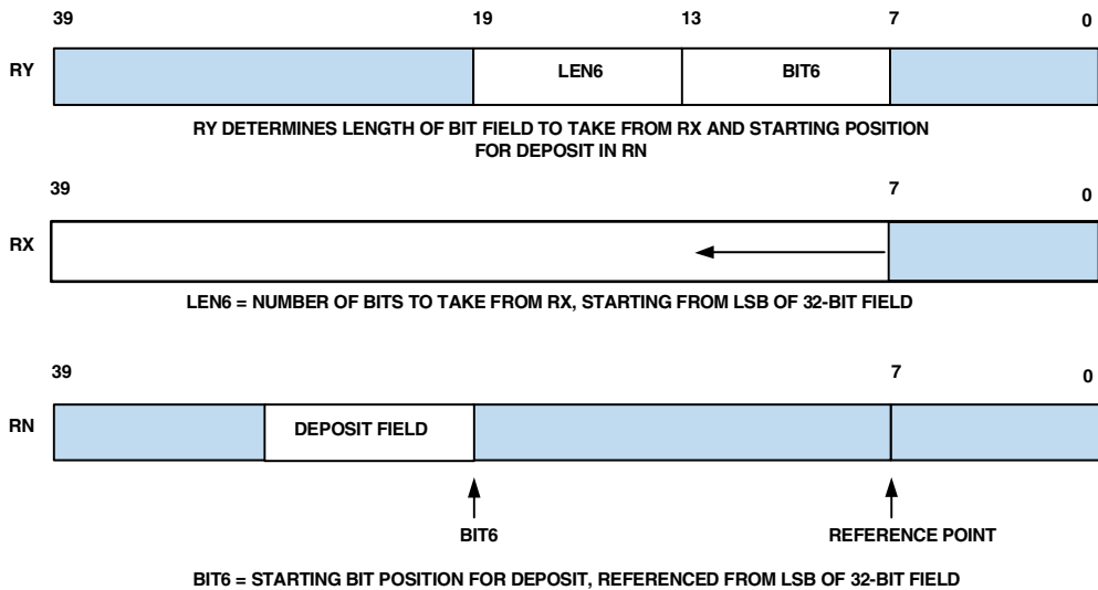
Figure 2-13. Bit Field Deposit Instruction
