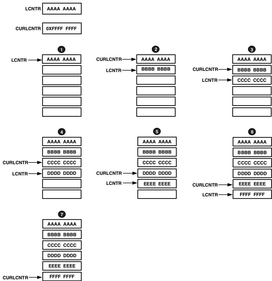
Figure 3-3. Pushing the Loop Counter Stack for Nested Loops
