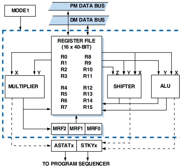
Figure 2-1. Computational Block
