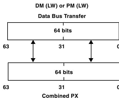
Figure 5-5. PX Register-to-Memory Transfers on PM Data Bus (LW)
