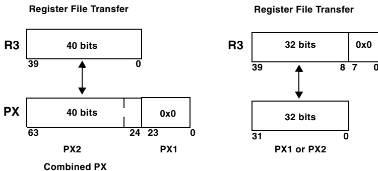
Figure 5-3. PX, PX1, and PX2 Register-to-Register Transfers
