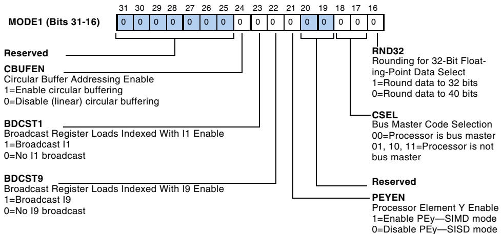
Figure B-1. Mode Control 1 Register Bits 31–16
