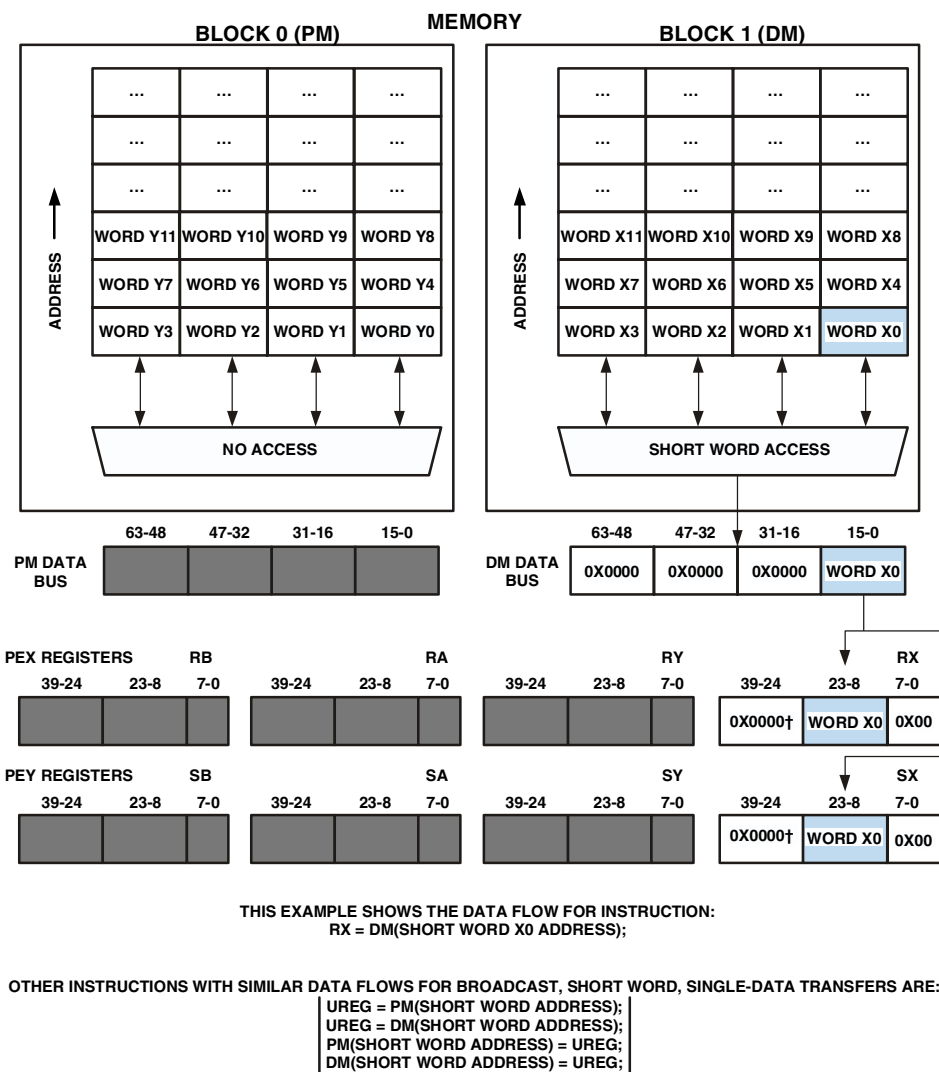
Figure 5-27. Short Word Addressing of Single-Data in Broadcast Load
