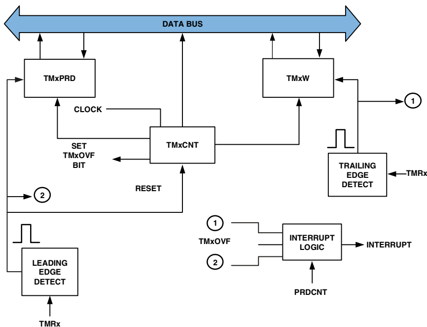
Figure 7-5. Timer Flow Diagram – WDT H _CAP Mode
