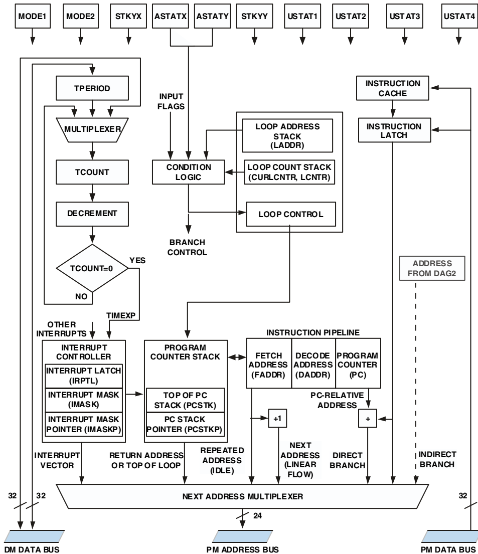
Figure 3-4. Program Sequencer Block Diagram
