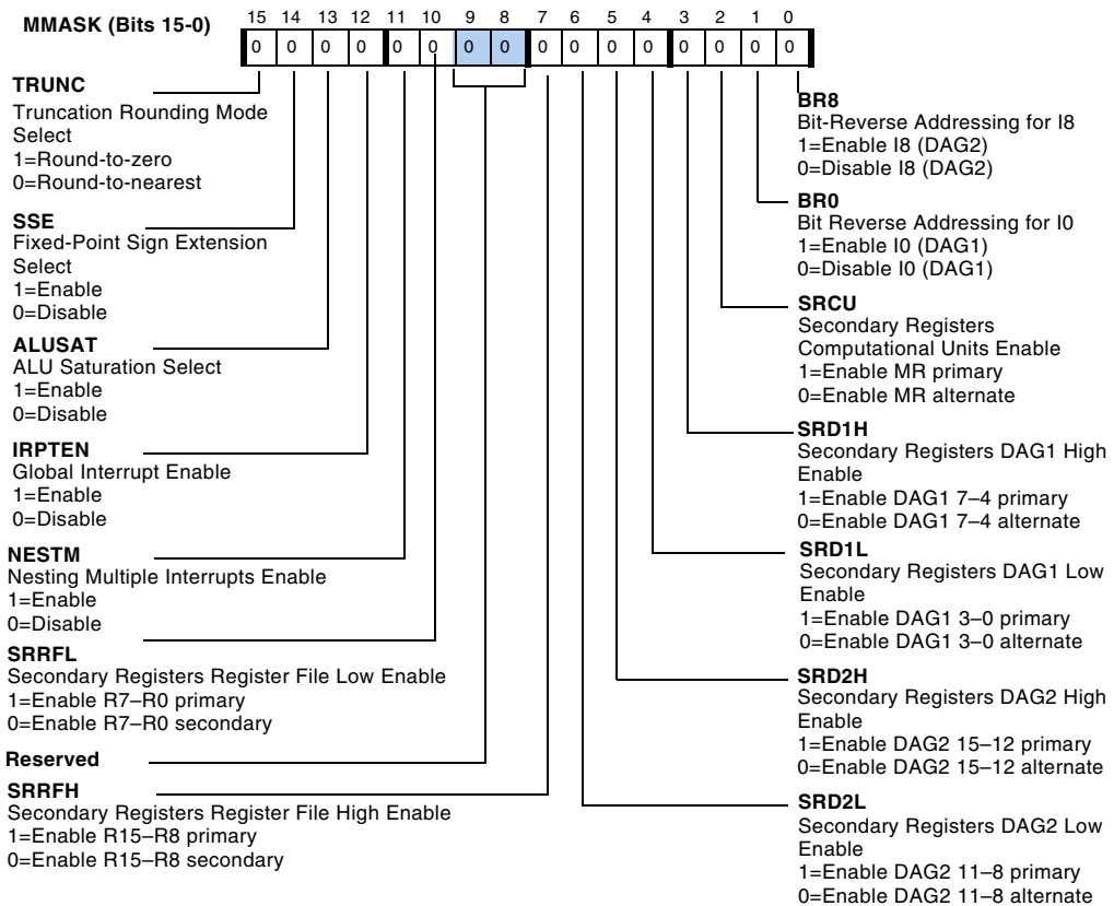
Figure B-4. MMASK Register Bits 15–0
