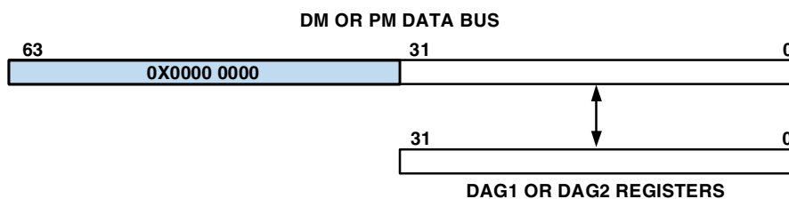
Figure 4-6. Normal Word (32-Bit) DAG Register Memory Transfers
