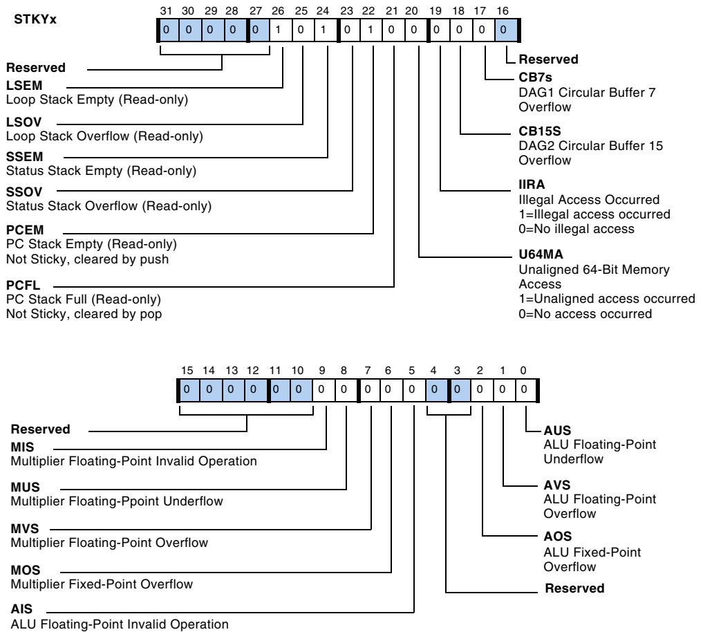
Figure B-8. STKYx Register
