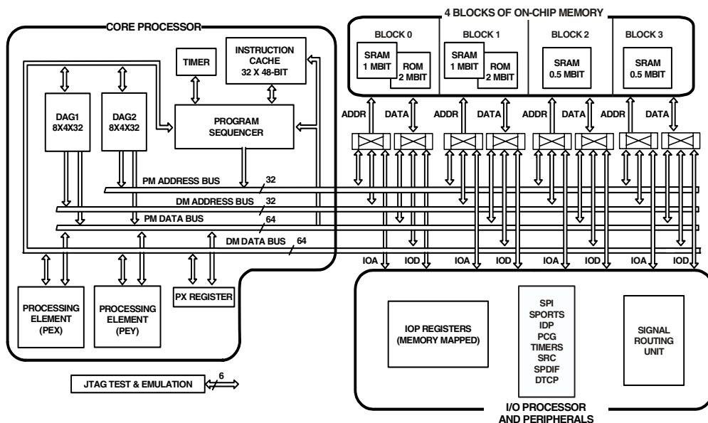
Figure 1-1. ADSP-21362/3/4/5/6 SHARC Processor Block Diagram
