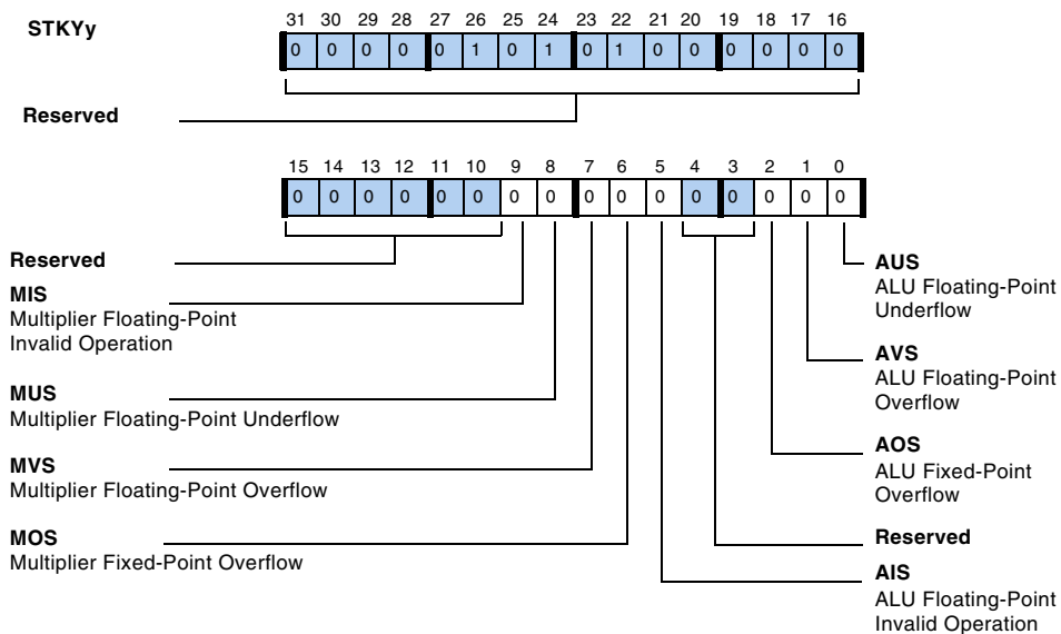
Figure B-7. STKYy Register
