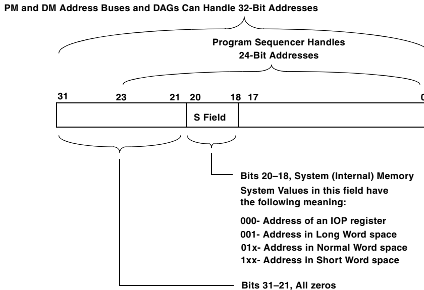
Figure B-11. PM and DM Bus Addresses Versus Sequencing Addresses
