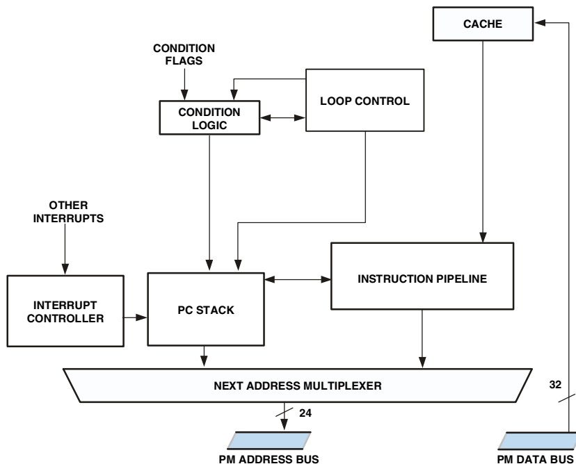
Figure 3-1. Program Sequencer Block Diagram
