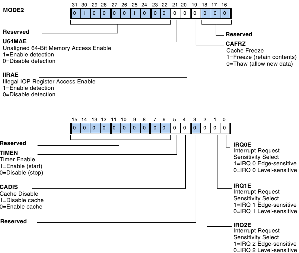
Figure B-5. MODE2 Control Register
