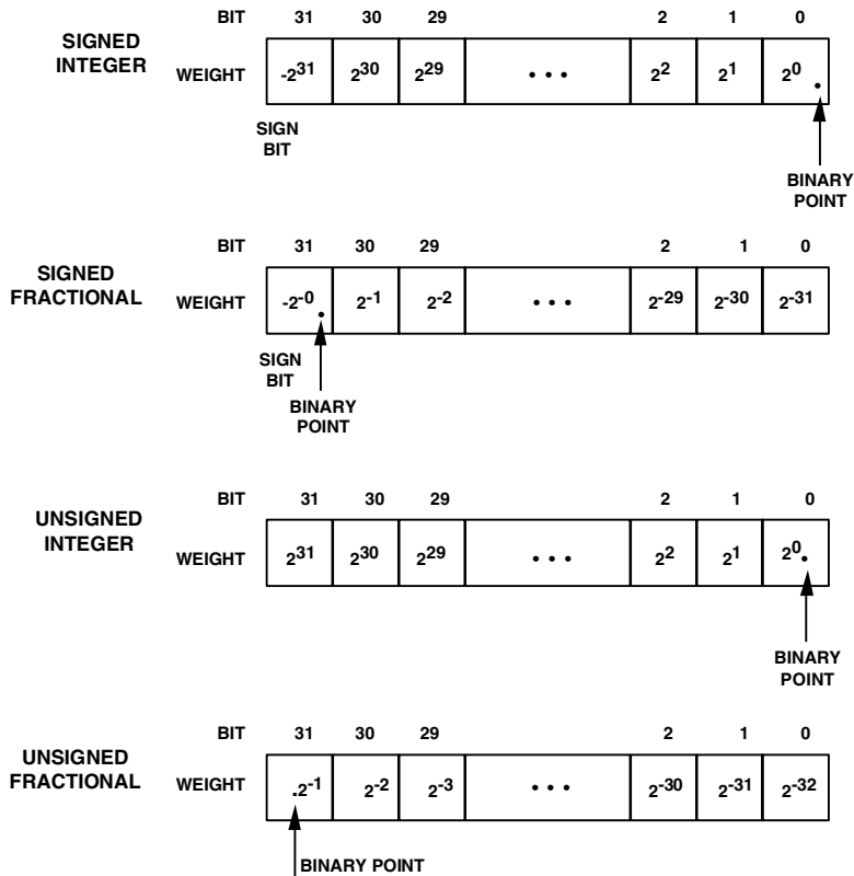
Figure 2-5. 32-Bit Fixed-Point Formats
