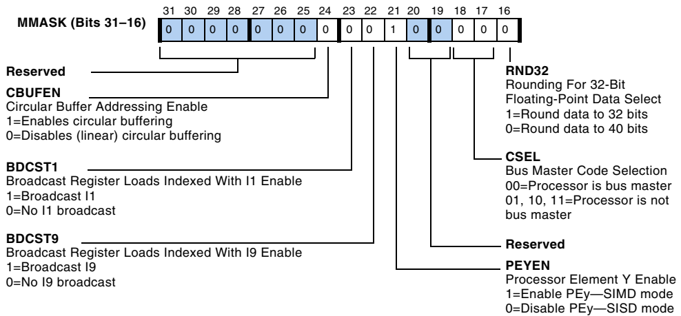
Figure B-3. MMASK Register Bits 31–16
