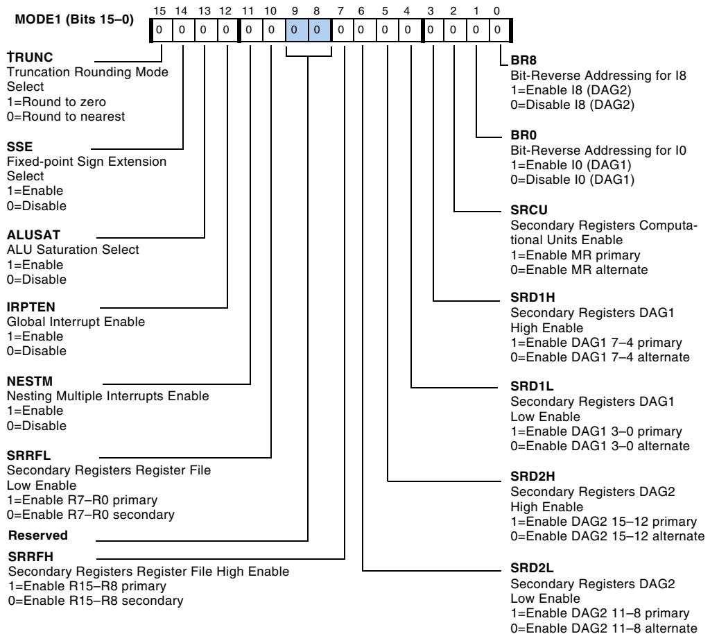
Figure B-2. Mode Control 1 Register Bits 15-0
