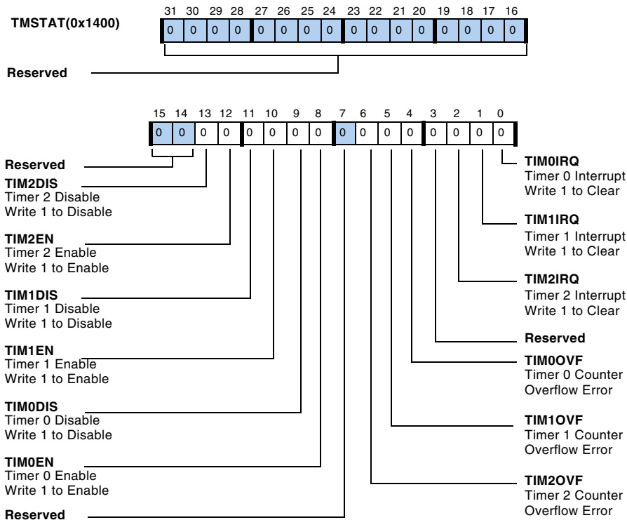
Figure B-13. TMSTAT Register
