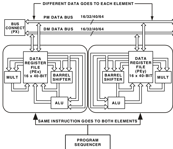
Figure 2-16. Block Diagram Showing Secondary Execution Complex
