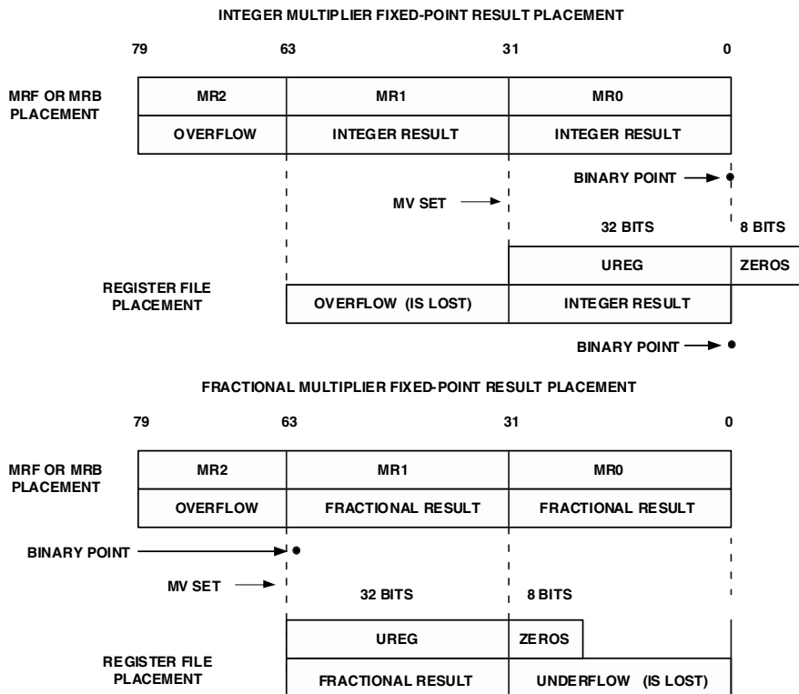
Figure B-9. MRFx and MRBx Registers
