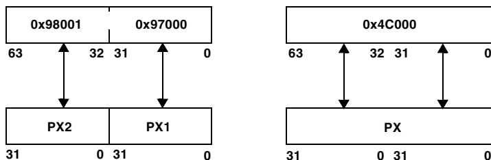
Figure 5-2. PM Bus Exchange (PX, PX1, and PX2) Registers
