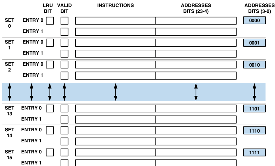
Figure 3-2. Instruction Cache Architecture
