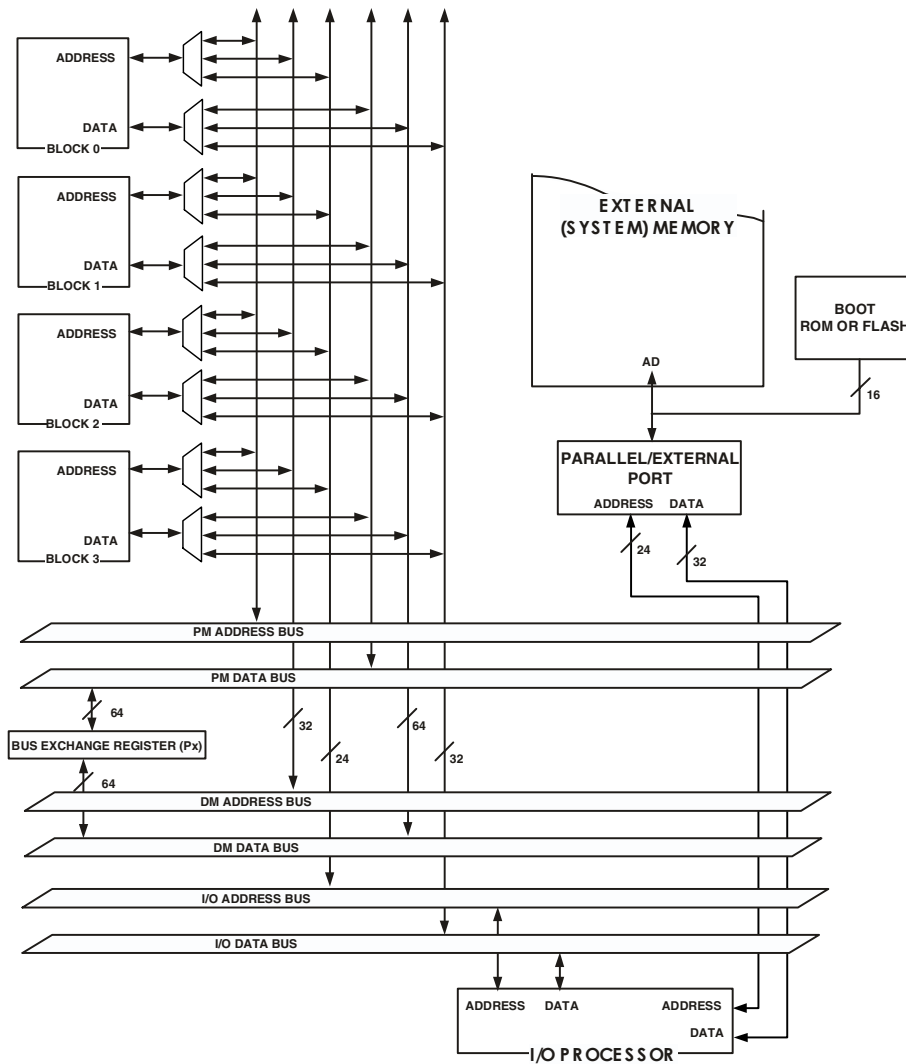
Figure 5-1. Memory and Internal Buses Block Diagram
