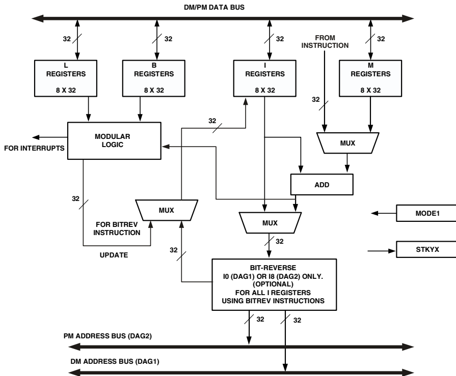
Figure 4-1. Data Address Generator (DAG) Block Diagram
