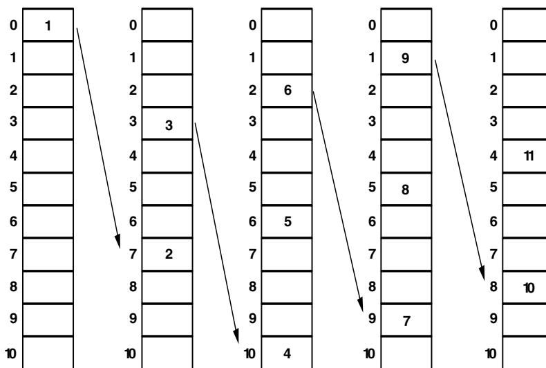
Figure 4-5. Circular Data Buffers With Negative Modifier
